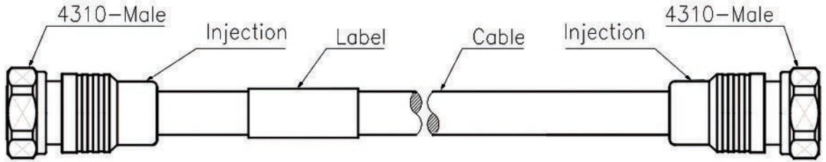
1/2" superflexible Jumper Assembly, 4.3-10 Screw type male to 4.3-10 Screw type male
