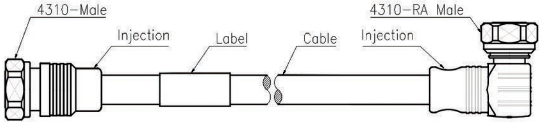
1/2" Flexible Jumper Assembly, 4.3-10 Screw type male to 4.3-10 Right angle Screw type male
