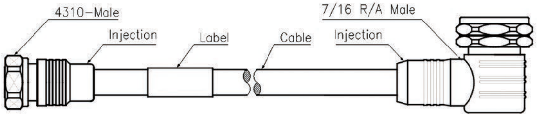
1/2" Flexible Jumper Assembly, 4.3-10 Screw type male to 7/16 Right angle type male
