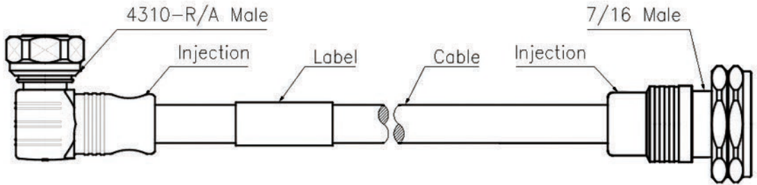
1/2" Flexible Jumper Assembly, 4.3-10 right angle screw type male to 7/16 type male
