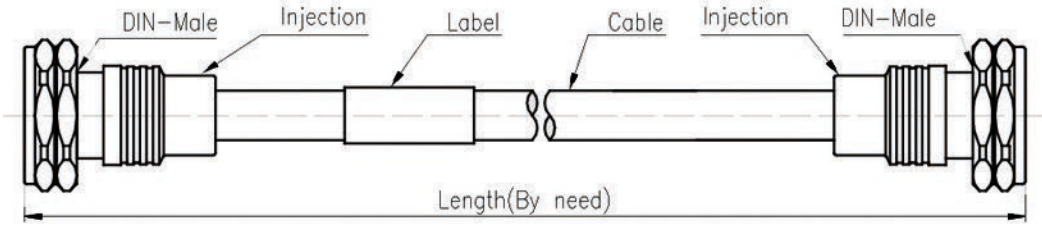
1/2" super flexible Jumper Assembly,DIN type male to DIN type male
