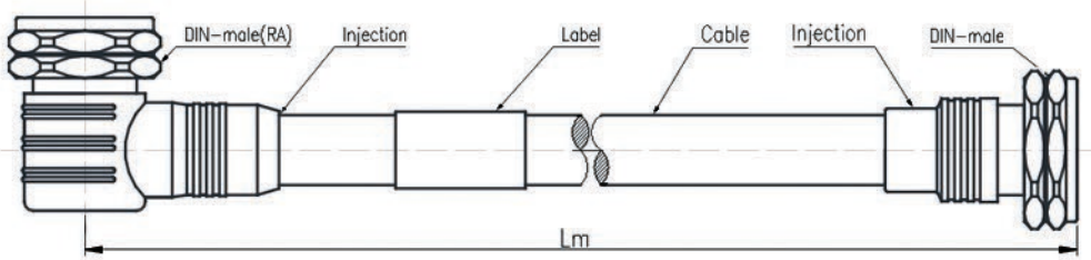
1/2" flexible Jumper Assembly, DIN type right angle male to DIN type male
